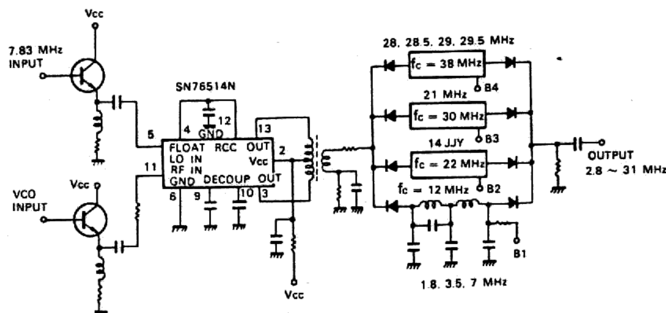
Second mixer circuit diagram
