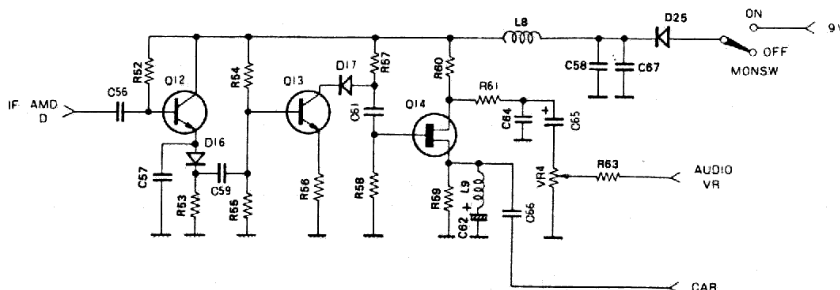
Fig. 5 Monitor circuitry
