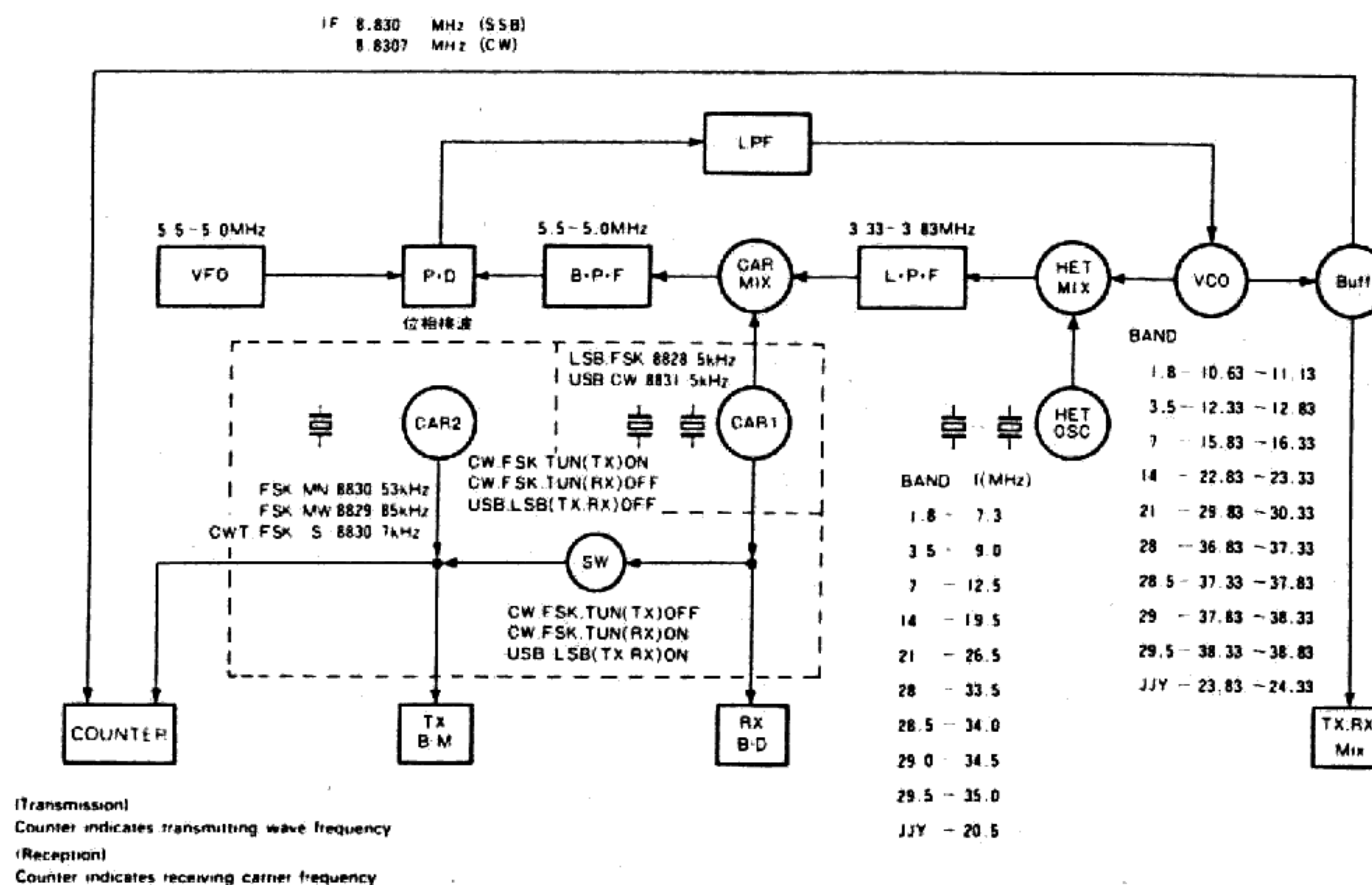
Fig. 6 PLL system
